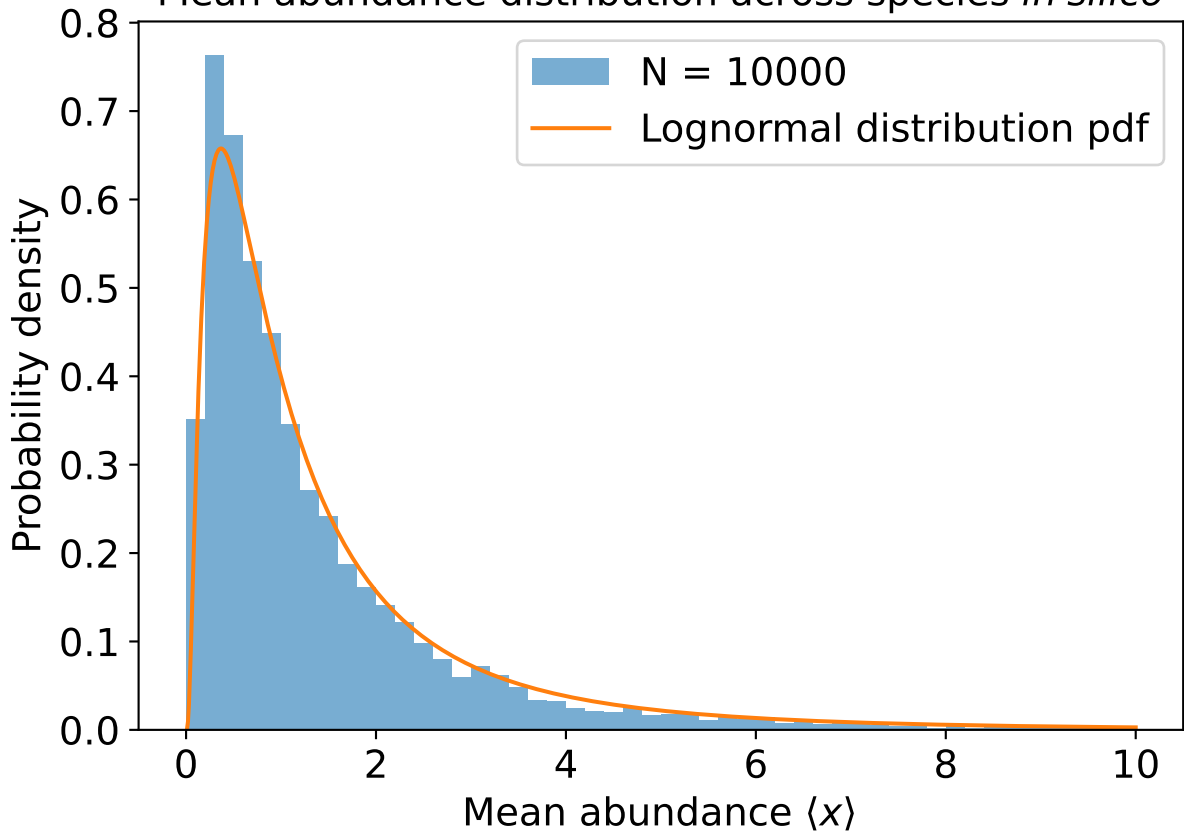
Mean abundance distribution across species in silico
